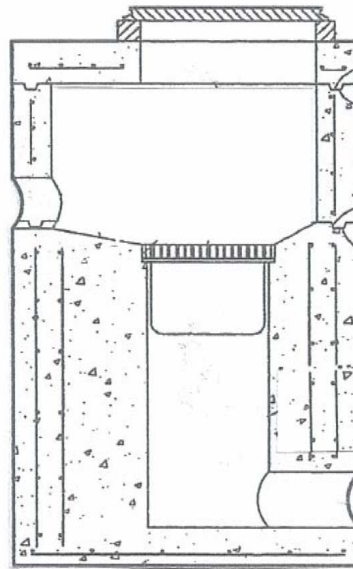
2. Side Outlet – GST001SO
