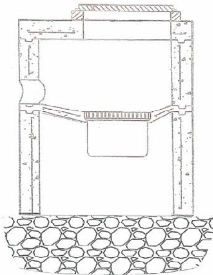
3. Disc Open Bottom – GST003DOB
