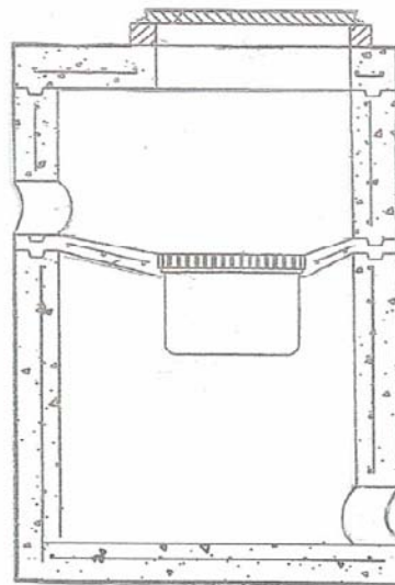
4. Disc Side Outlet – GST004DS
